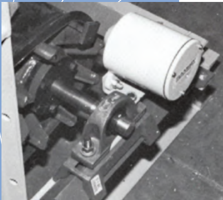
△ Under Speed Switch in Rotating Equipment ▷ Model 60-23P
